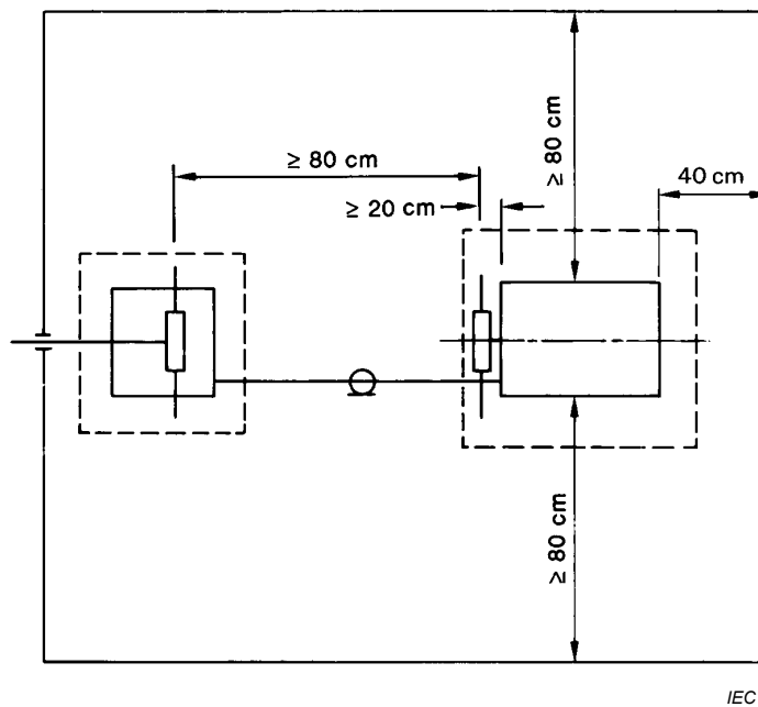
Figure 6 – Measurement of the radiofrequency disturbance voltage injected into the mains (top view) (see 5.3.1)
